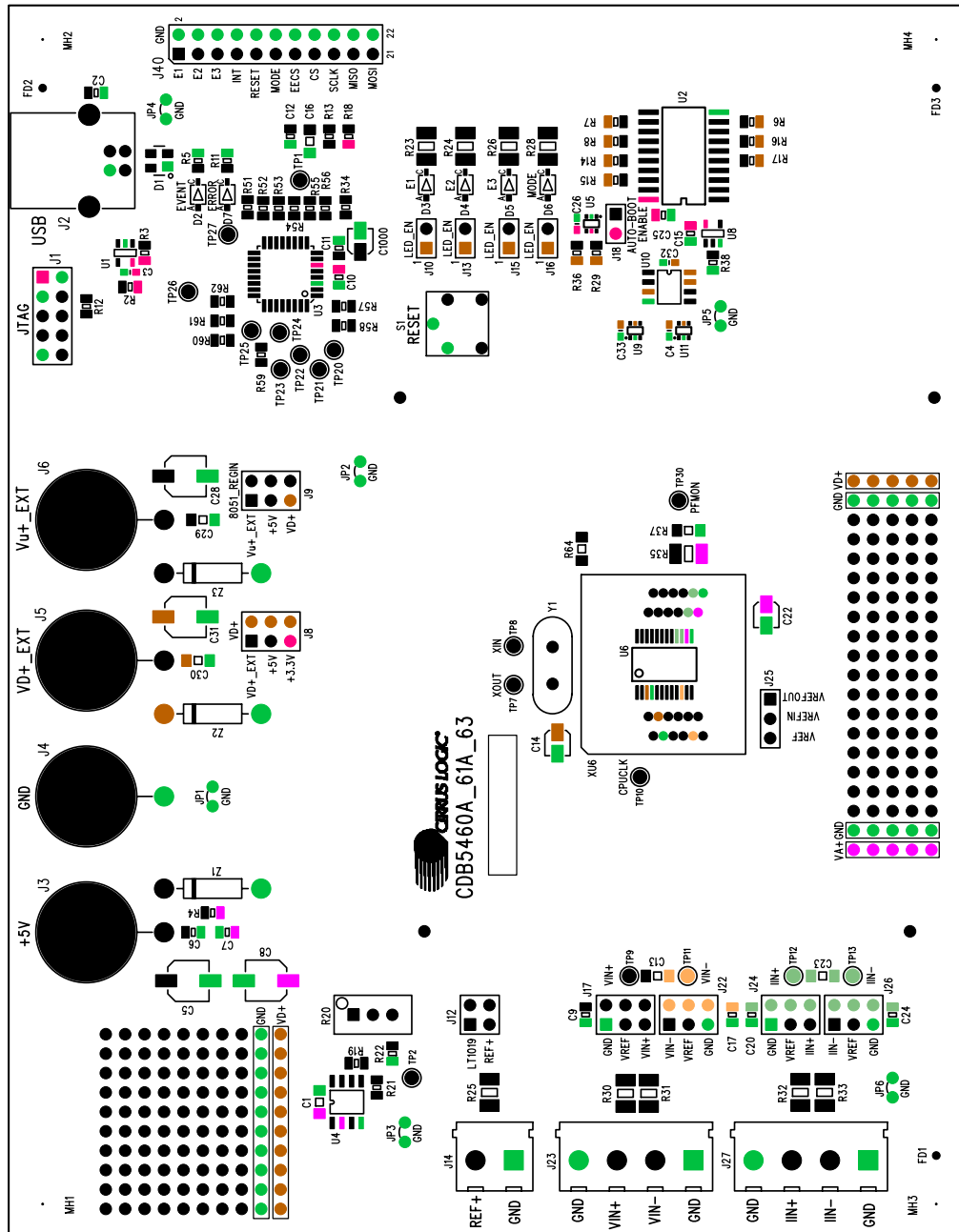
CIRRUS LOGIC PC-240-00176-Z1 Rev B SILKSCREEN TOP
